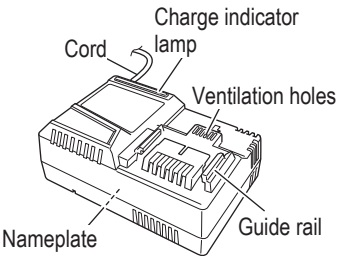
<UC18YSL3> Fig. 4
