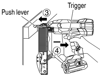
Stapling operation switch
